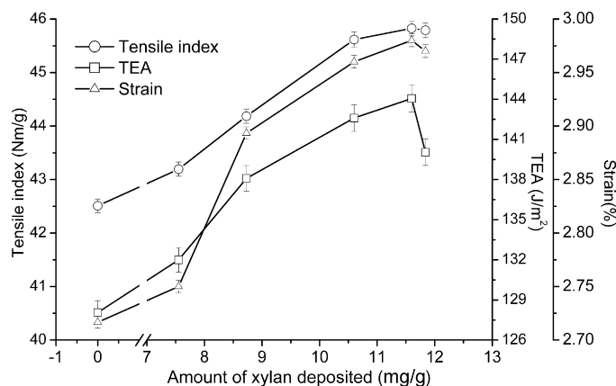
Fig. 2. Effect of xylan addition on tensile index.
