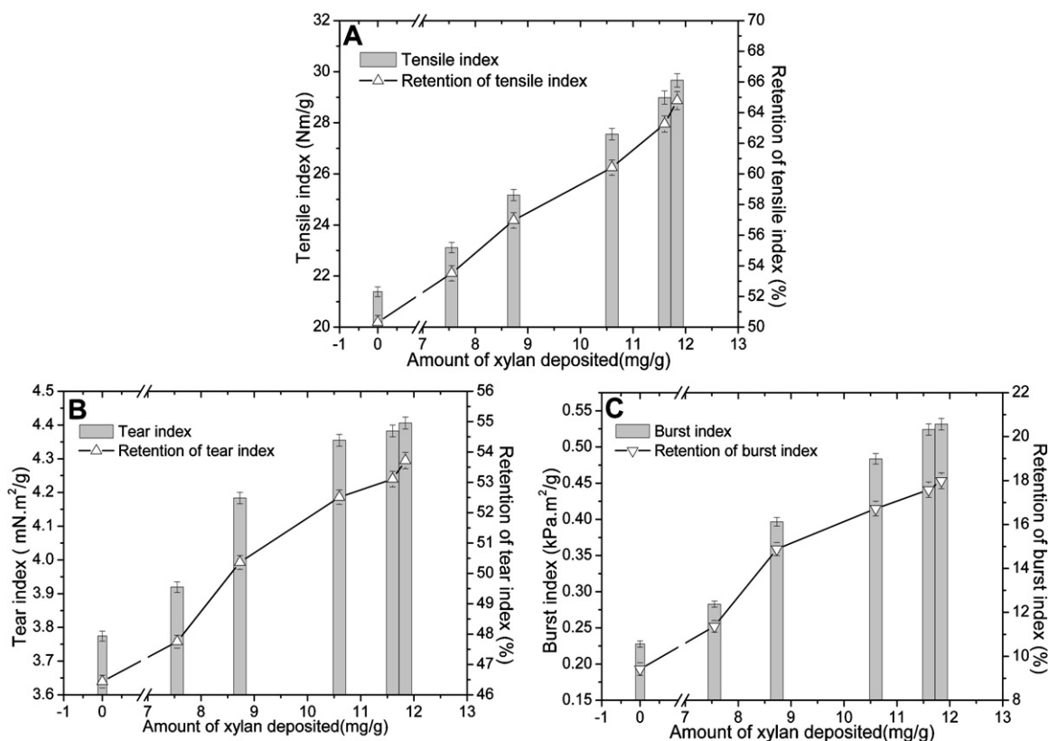
Fig. 4. Effect of xylan addition on tensile (A), tear burst (B), and burst (C) after drying.
