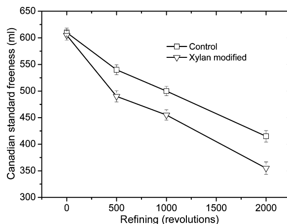
Fig. 5. Effect of xylan on the PFI refining.
