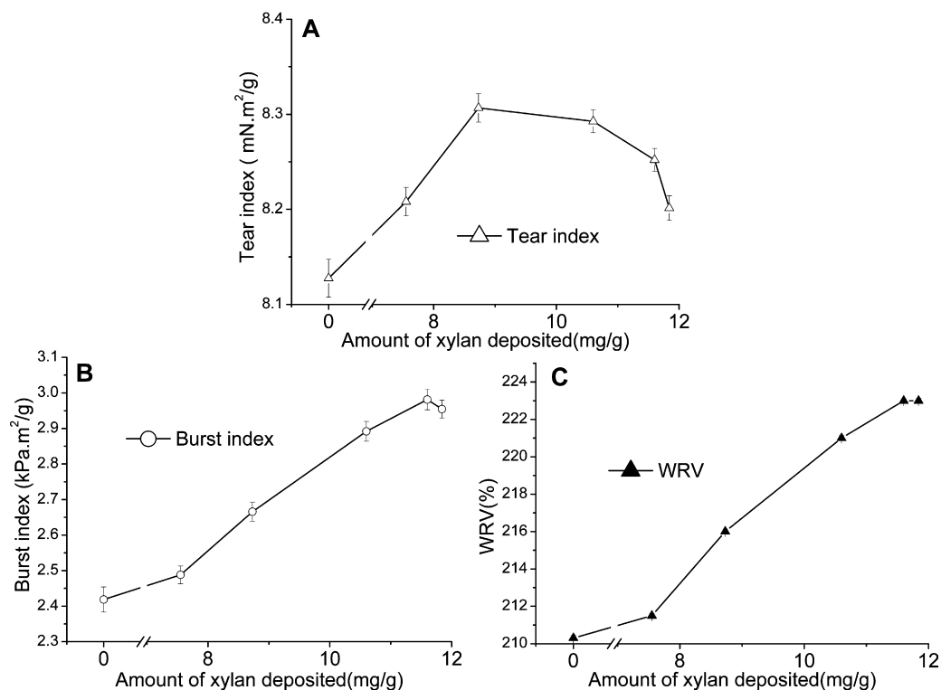
Fig. 3. Effect of xylan addition on tear (A), burst (B), and WRV (C).
