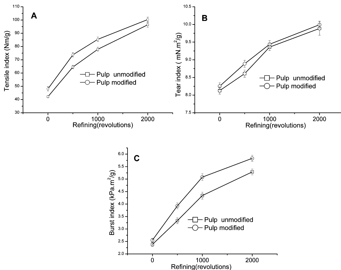
Fig. 6. Effect of refining on the mechanical properties.
